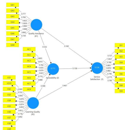
Fig. 2. Model Outer Loading
